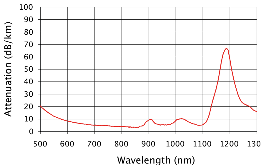
Typical Attenuation
